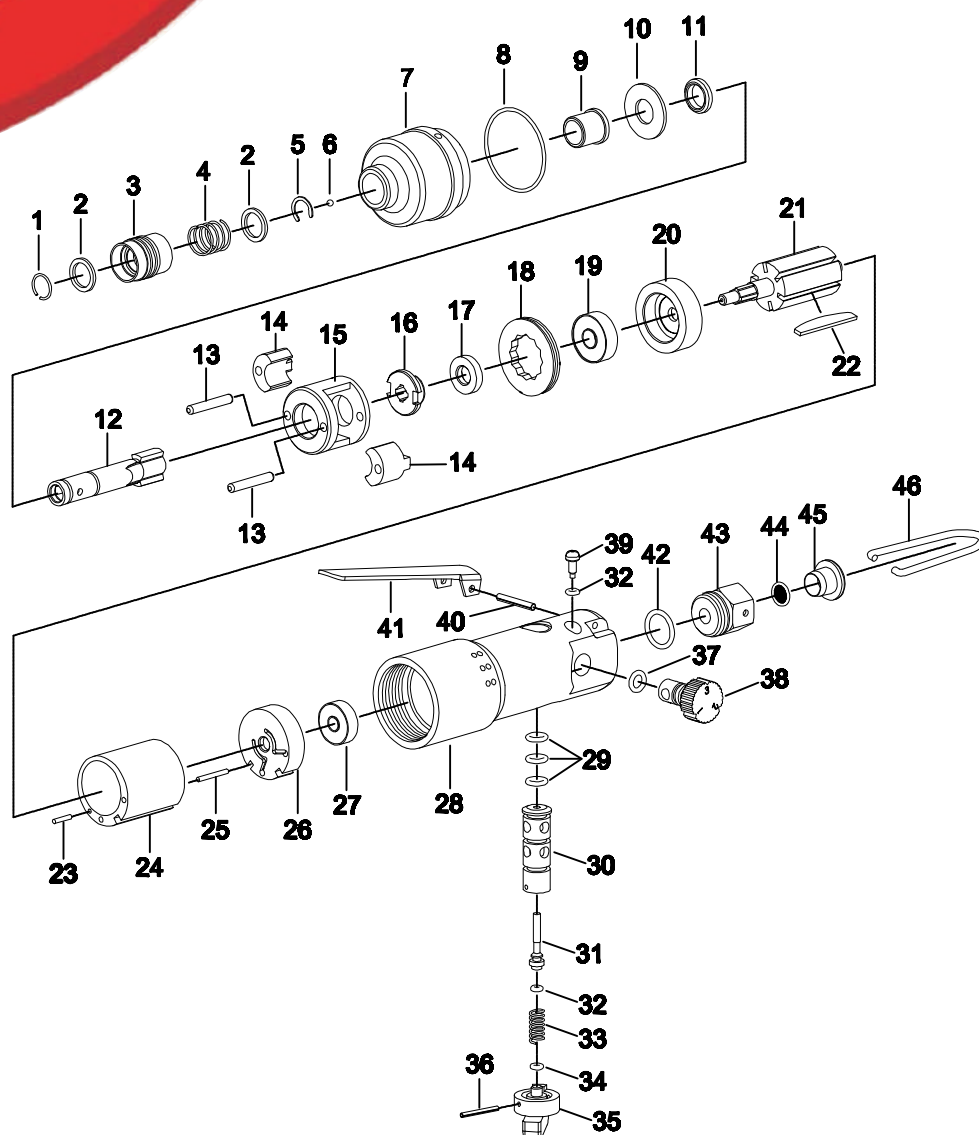
Exploded View
